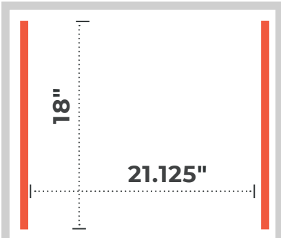
5" DEPTH CHAMBER CAPACITY
